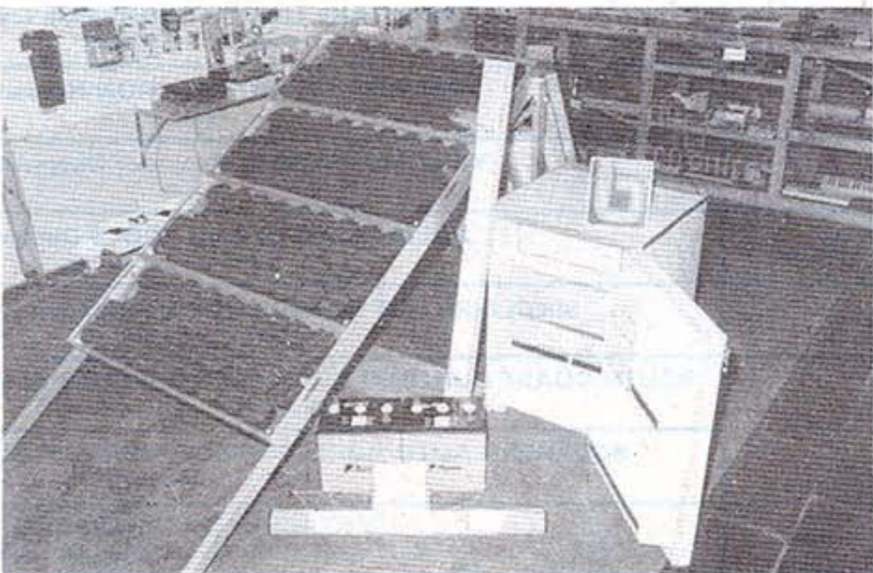
AN advanced solar powered fridge and lighting plant. Sunlight is converted into 12 volts at 10amps (120 watts) which charges the special batteries. The system is complete with charge regulator and high efficiency fluorescent lights. If you're into off roading, camping, boating or remote dwellings here is your freedom! South East Electronics provides full design and installation services to solve your energy problems—see us today.
